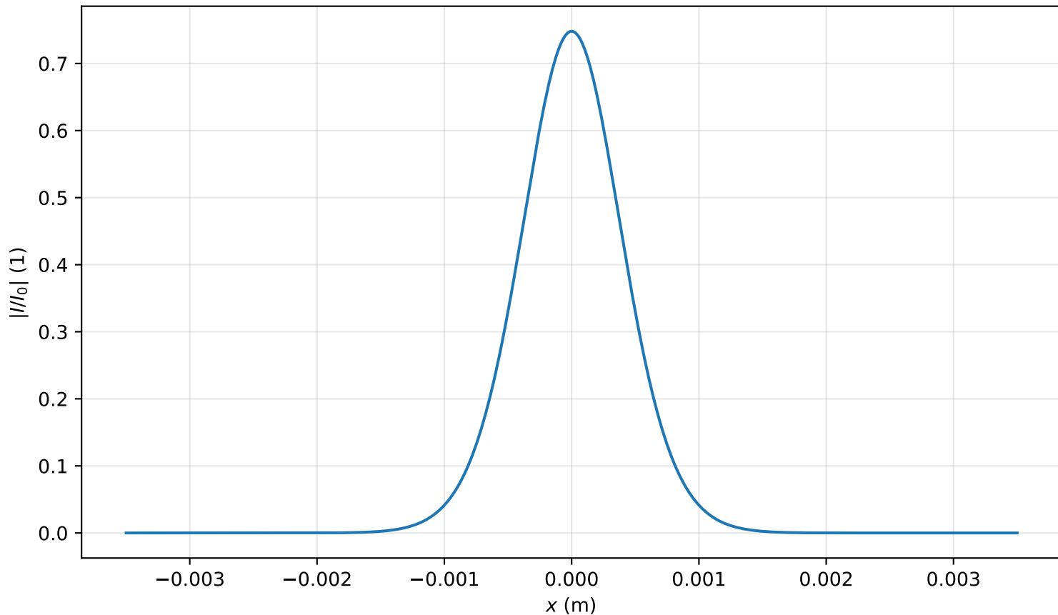
Intensity profile I(x, y = 0, z = 1.672m)/I_0 , P_{in}=0.3P_{cr} , artificial time
